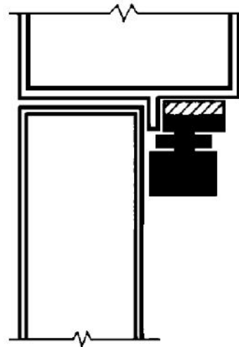
Figure 4 Jamb bracket shim for blade stop doors 明装顶置门止：叶片止口安装
