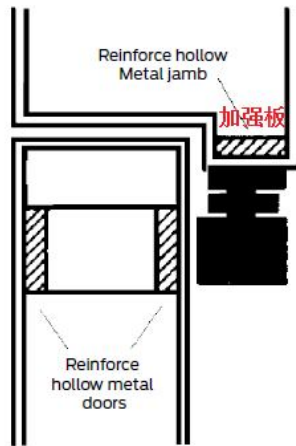
Figure 1 Typical installation 明装顶置门止：经典安装
