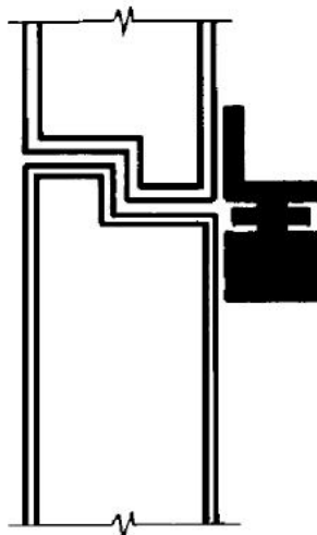
Figure 3 Angle jamb bracket for flush transom or rabbeted doors 明装顶置门止：其扼门角码安装
